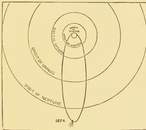
FIG. 99.—Orbit of Halley's comet.
